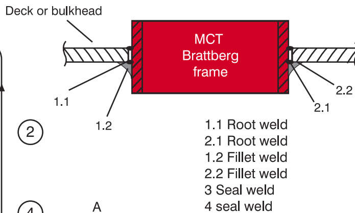
FIG 4: Welding sequence
