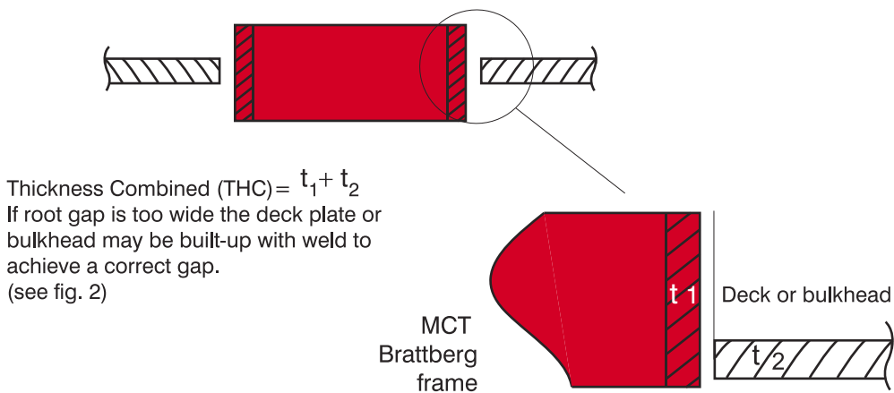
FIG 1: maximum allowable root gap for fillet joint
