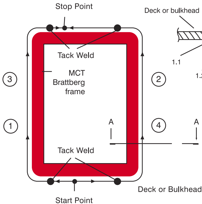
FIG 4: Welding sequence
